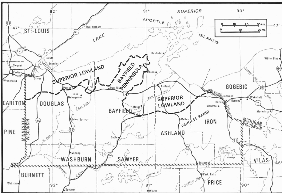
Figure 2: Superior Region (Clayton, 1984)
