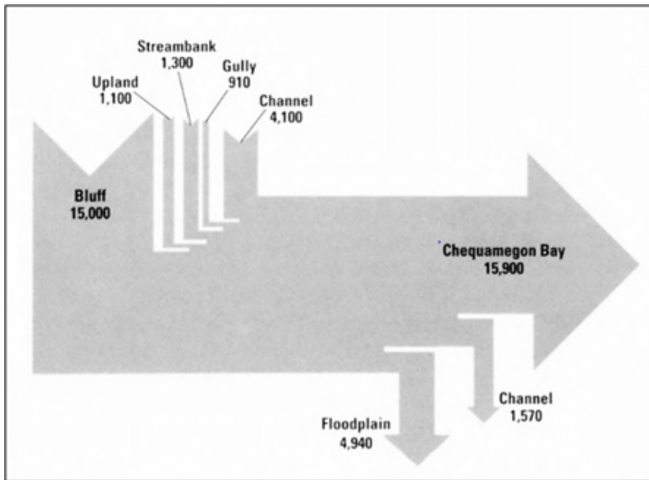
Figure 11: Historical Annual Sediment Budget For North Fish Creek In Metric Tonnes Per Year.
