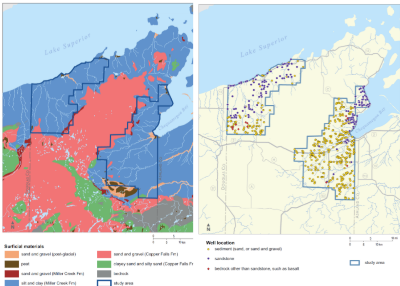
Figure 17: The Study Area Along With Surficial Geologic Deposits And Well Construction.
