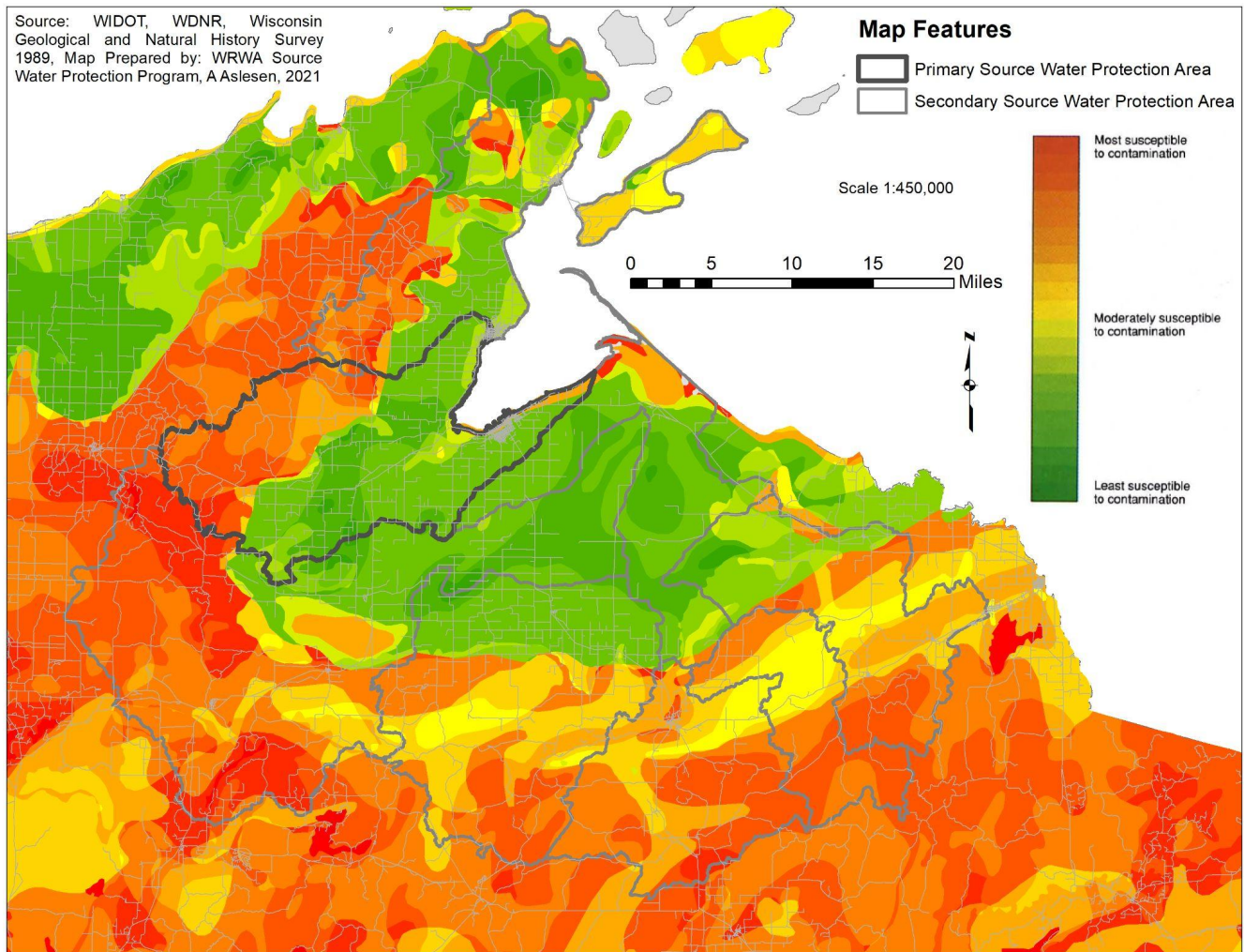
Figure 16: Map of groundwater contamination susceptibility in the primary and secondary watersheds.
